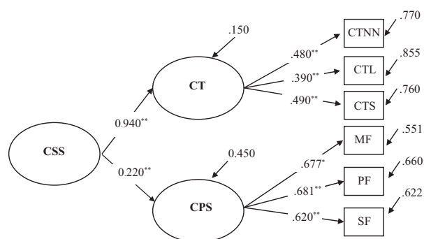
Figure 1 Confirmatory factor analysis of grade 9 students' cognitive skill mode
