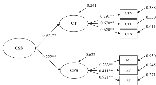
Figure 2 Confirmatory factor analysis of grade 12 students' cognitive skill mode
