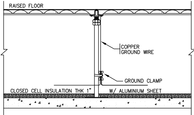
DETAIL FOR GROUND GRID INSTALLATION
