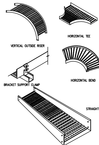
CABLE TRAY DETAIL
