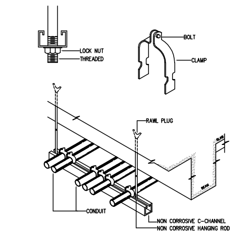
CONDUIT SUPPORT DETAIL.
