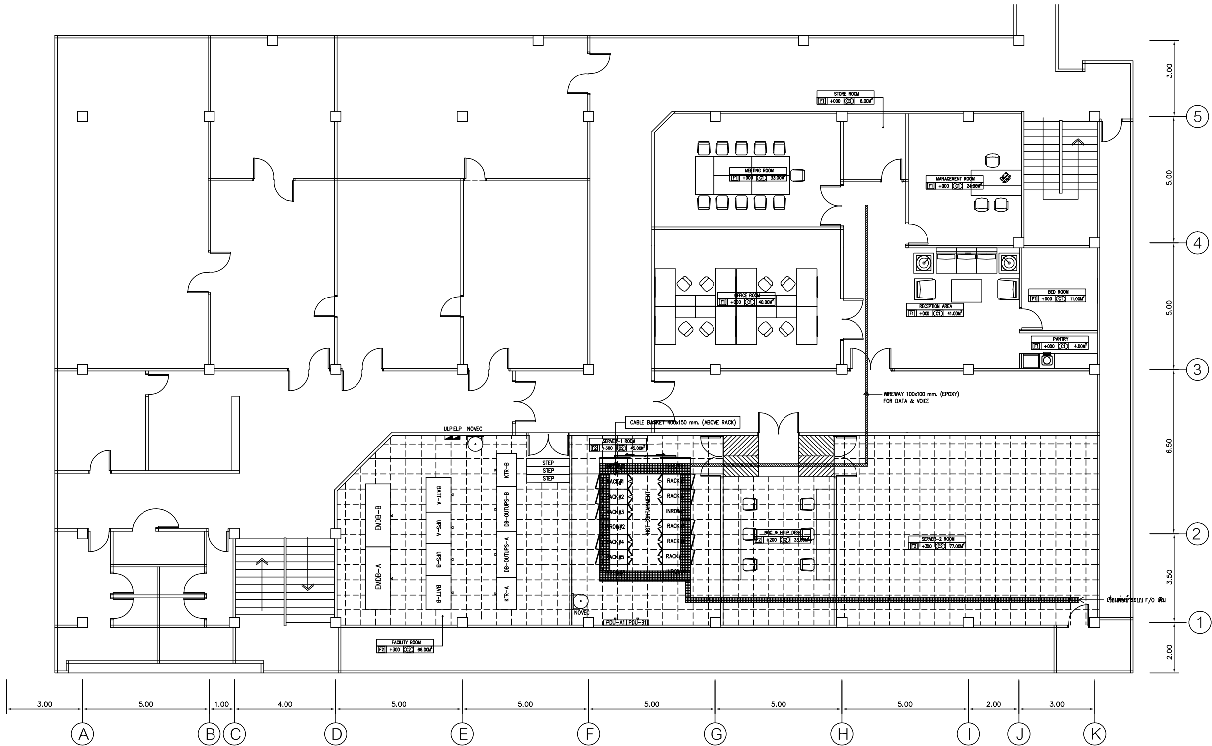
CABLE BASKET LAYOUT SCALE 1 : 75
