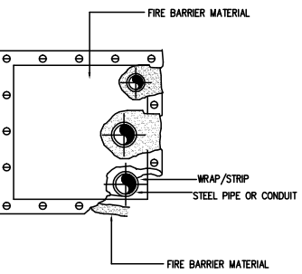
PIPING THROUGH FIRE WALL AND FLOOR DETAILS
