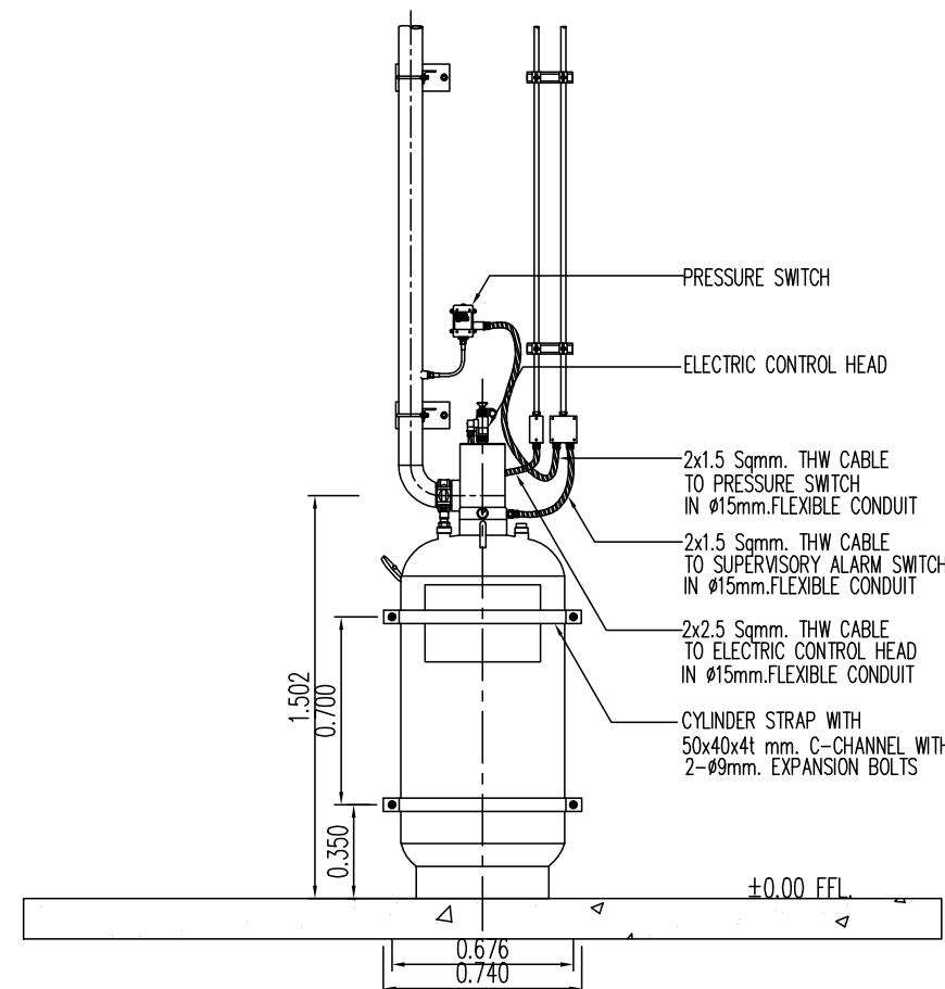
NOVEC-1230 CYLINDER INSTALLATION DETAIL
