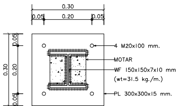
section 1-1 SCALE 1:7.5
