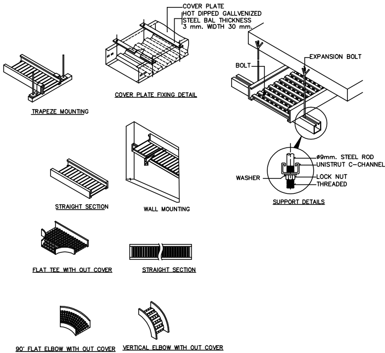
CONDUIT AND CABLE TRAY INSTALLATION AND SUPPORT
