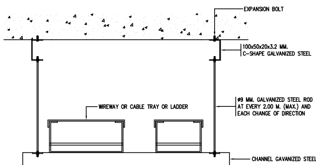
CABLE TRAY SUPPORT DETAILS
