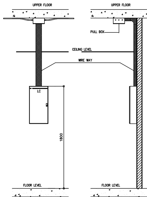
LOAD CENTER INSTALLATION DETAIL
