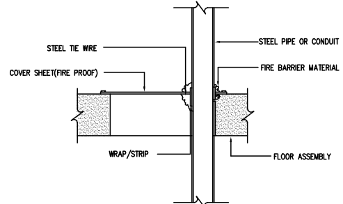
CABLE TRAY THROUGH FIRE WALL AND FLOOR DETAILS
