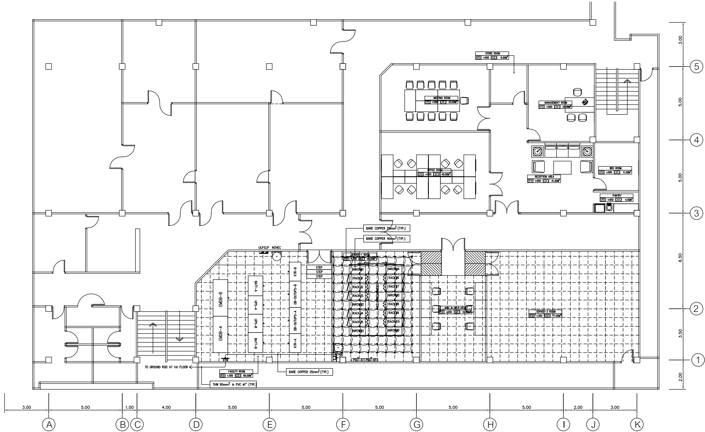
SIGNAL REFERENCE GROUNDGRID LAYOUT SCALE 1 : 75
