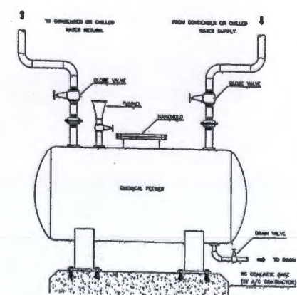
BY-PASS CHEMICAL FEEDER
