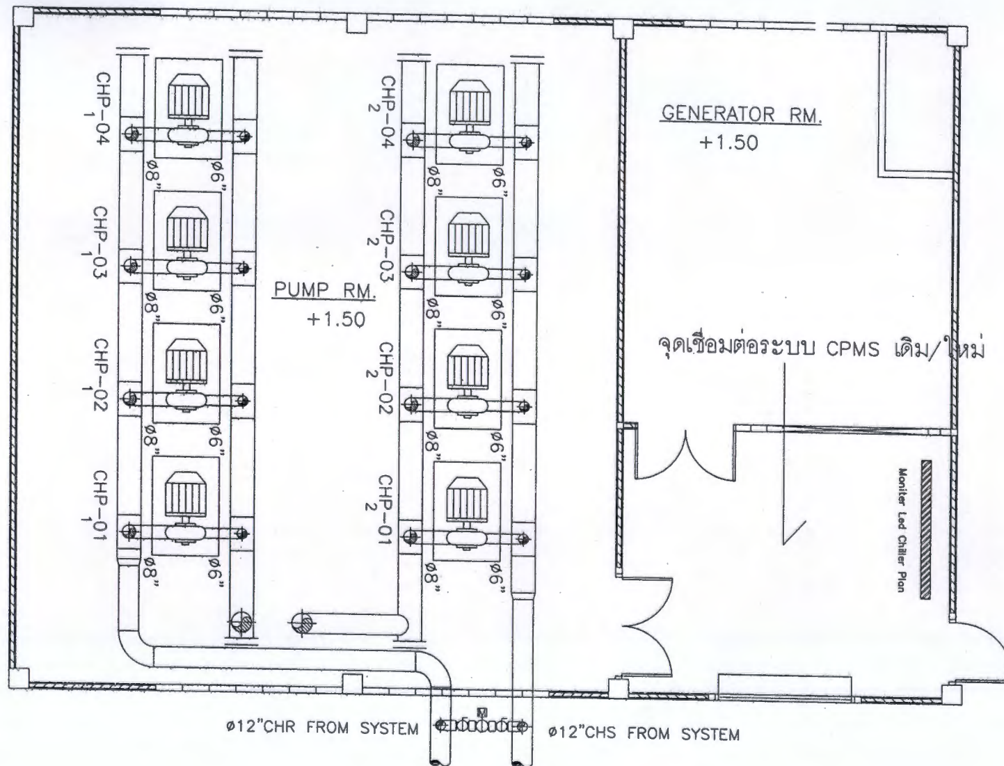
SECTION PUMP
