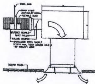
SQUARE CEILING DIFFUSER
