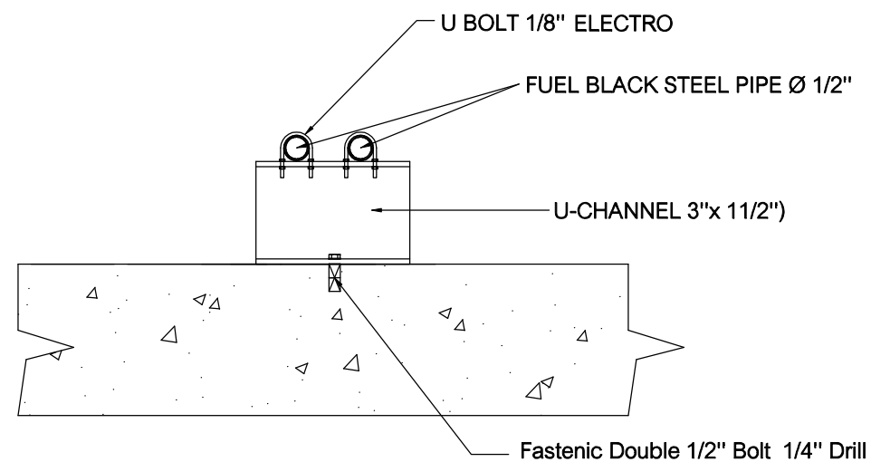
INSTALLATION FUEL PIPE
