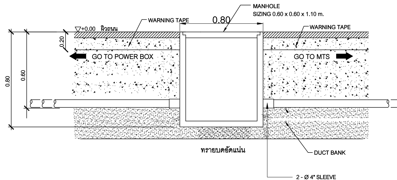
DETAIL DUCT BANK UNDERGROUND
